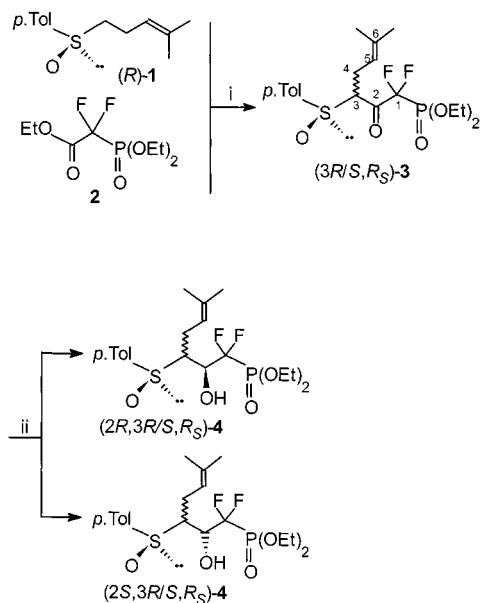
Scheme 2. Reagents and conditions: (i) LDA, THF, -70°C; (ii) NaBH 4 , CH 3 OH/NH 3 , 0°C
